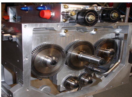
>> Fully balanced bottom end
