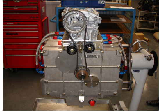
›› DI-3 multi cylinder head mounted on high speed bottom end
